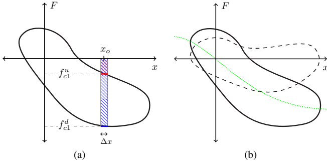
Fig. 2: a: Calculating work from force-displacement graph.
